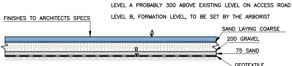
3 PATH SECTION SCALE 1:50
